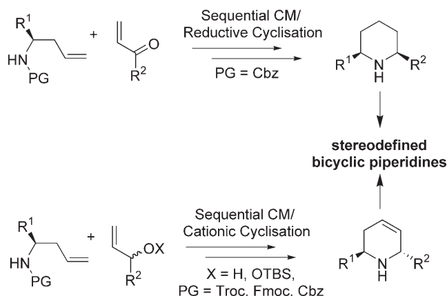
Scheme 1. CM cyclisation sequences (PG = protective group).
