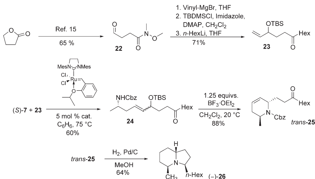
Scheme 2. Total synthesis of indolizidine enantiomer (–)- 26 .
